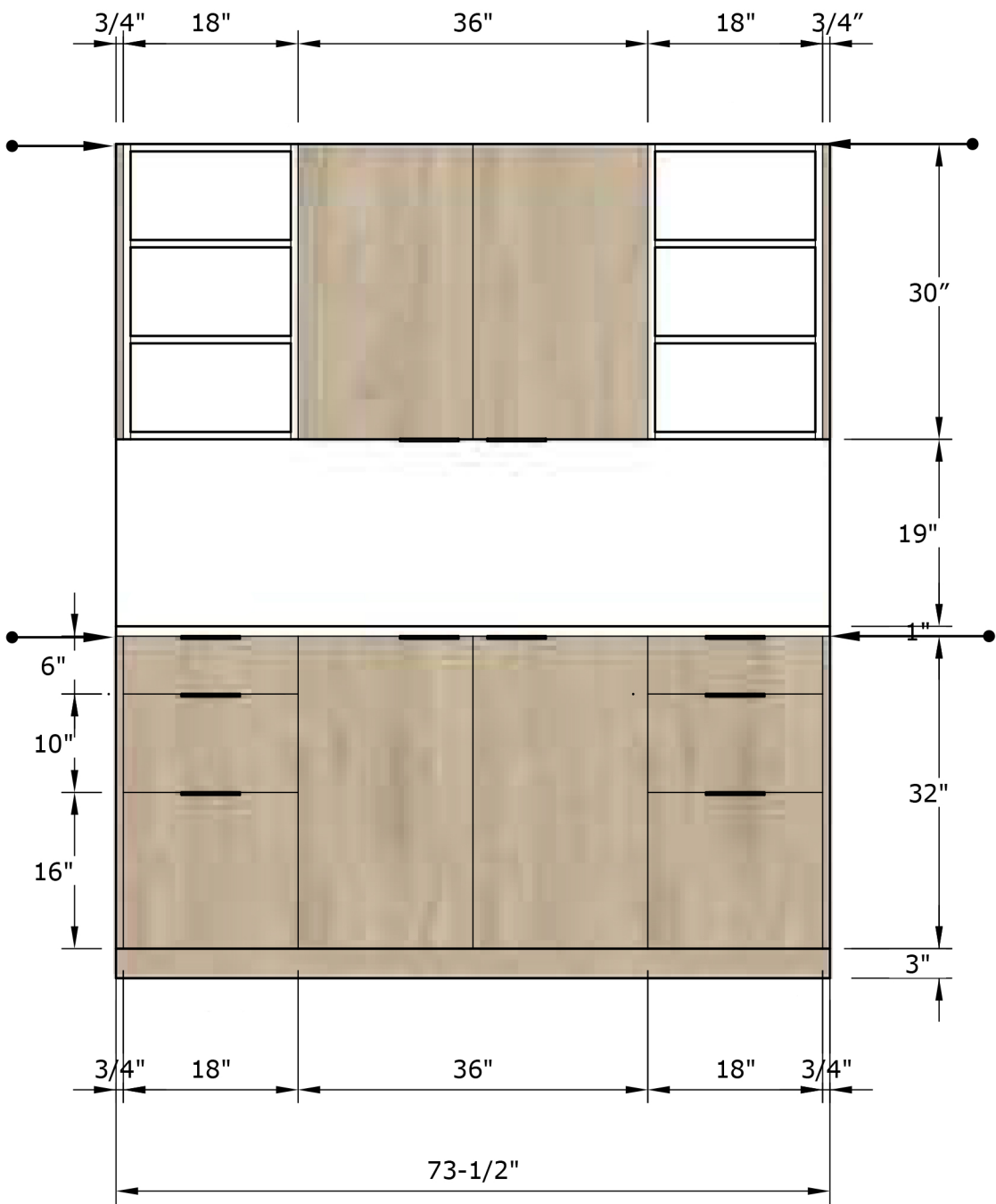
2 Front Elevation
