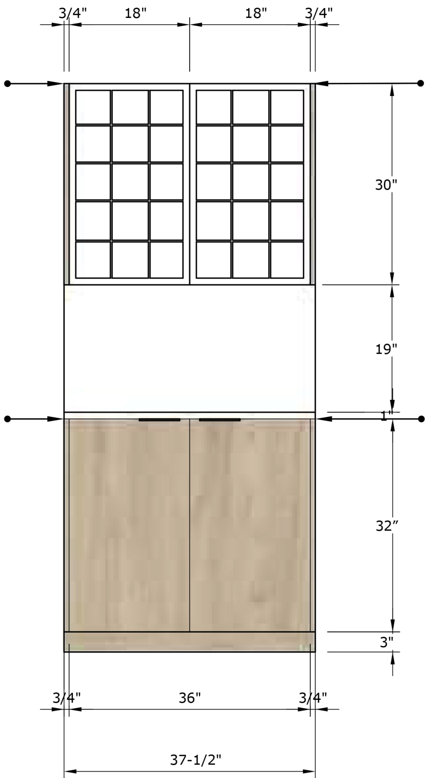
2 Front Elevation
