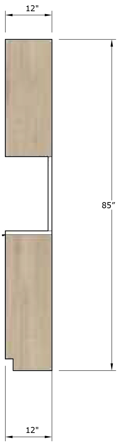
3 Side View
